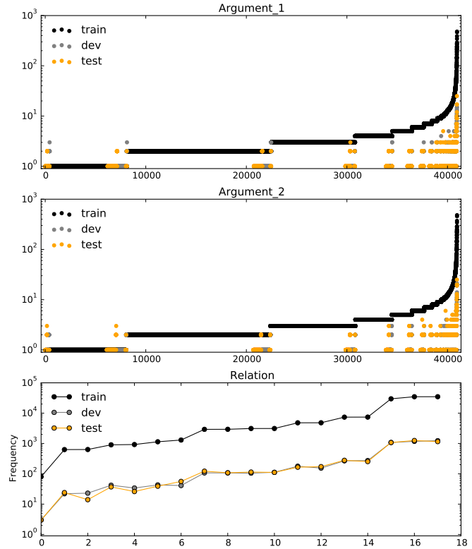
Figure 2: WordNet18 dataset frequency statistics
